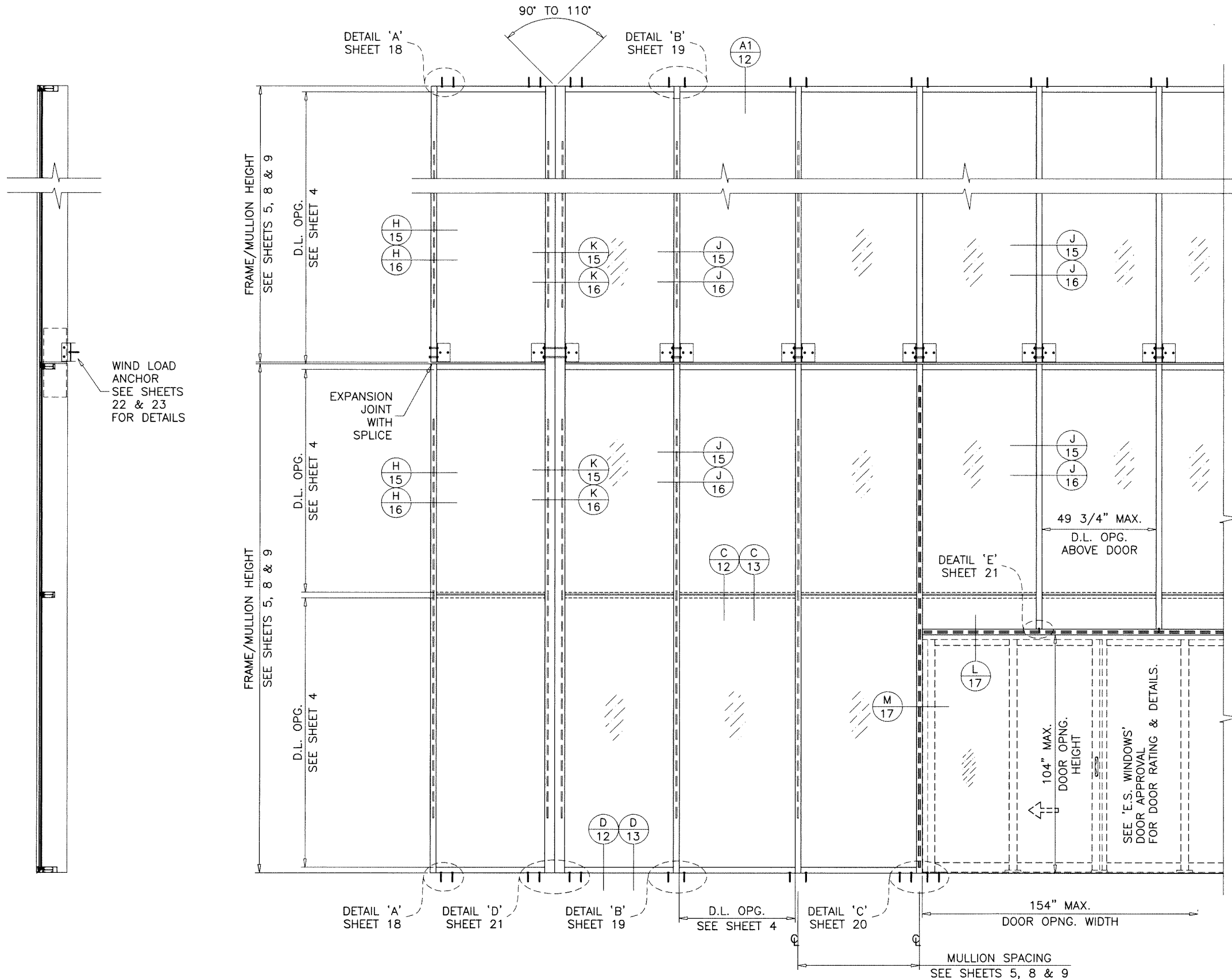
TYPICAL ELEVATION TWIN SPAN WITH 90° OR 110° EXTERIOR CORNERS (OPTIONAL TOP LOUVERS NOT SHOWN)
