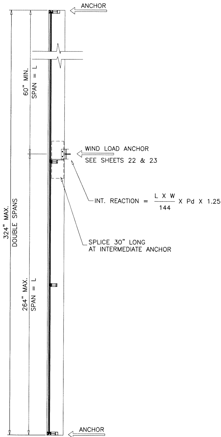
DOUBLE SPANS
