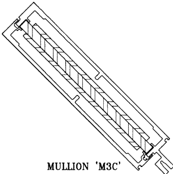
MULLION 'M3C'
