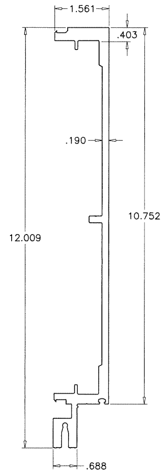
E7 MALE MULLION
